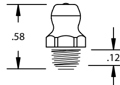
1/4"-28 SPECIAL TAPER THD. (Recommended hole size-.230 to .235")
