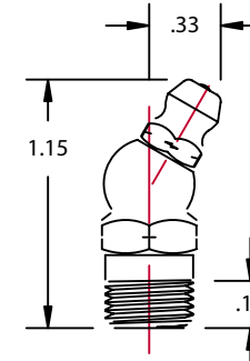
1/8" PTF SAE SPL SHORT
