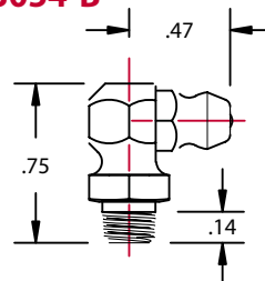
1/4"-28 SPECIAL TAPER THD. (Recommended hole size-.230 to .235")
