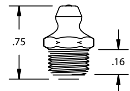
1/8" SAE SPL EXTRA SHORT
