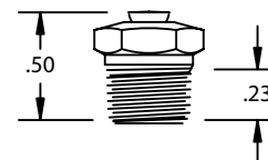
1/8" BSPT RELIEF FITTING
