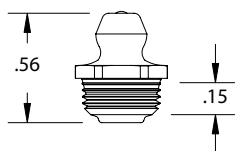
1/8" PTF SAE SPL EXTRA SHORT
