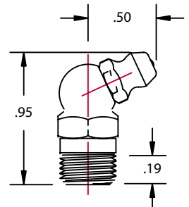
1/8" PTF SAE SPL SHORT
