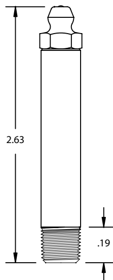
1/8" PTF SAE SPL SHORT
