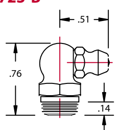
1/8" PIPE SPECIAL TAPER THD. (Recommended hole size-.373 to .380")
