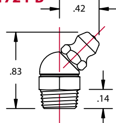
1/8" PIPE SPECIAL TAPER THD. (Recommended hole size-.373 to .380")
