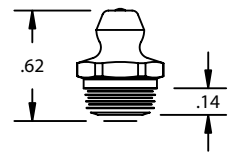
1/8" PIPE SPECIAL TAPER THD. (Recommended hole size-.373 to .380")
