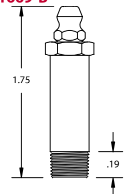
1/8" PTF SAE SPL SHORT
