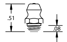
1/4"-28 SPECIAL TAPER THD. (Recommended hole size-.230 to .235")
